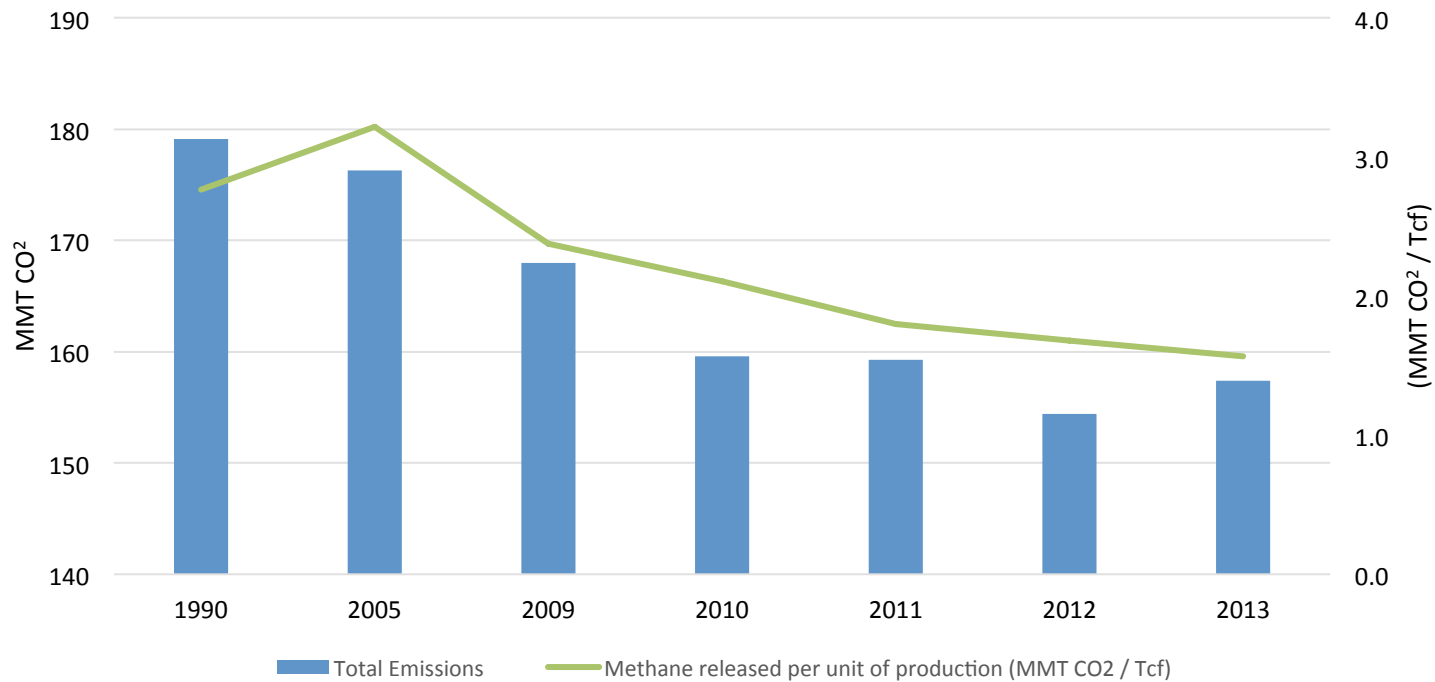
Natural Gas Methane Emissions Per Unit of Production (MMT CO 2 /Tcf)
