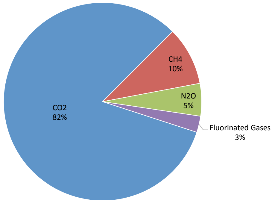
U.S GHG Emissions: 2013 MMT CO 2 equivalent
